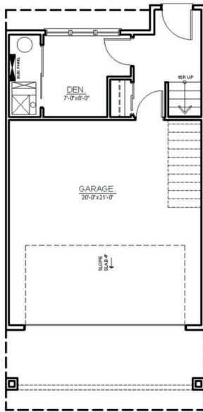
LOWER FLOOR 200 SQFT.
