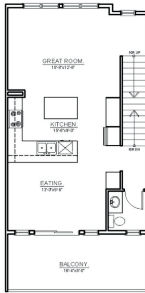
MAIN FLOOR 643 SQFT.
