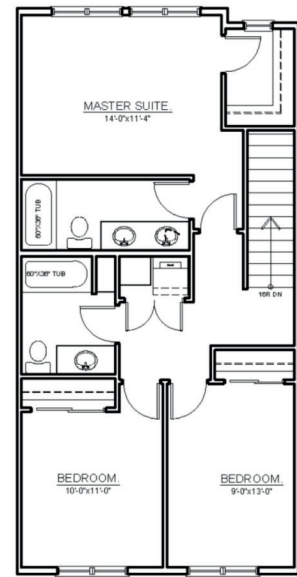
UPPER FLOOR 805 SQFT.
