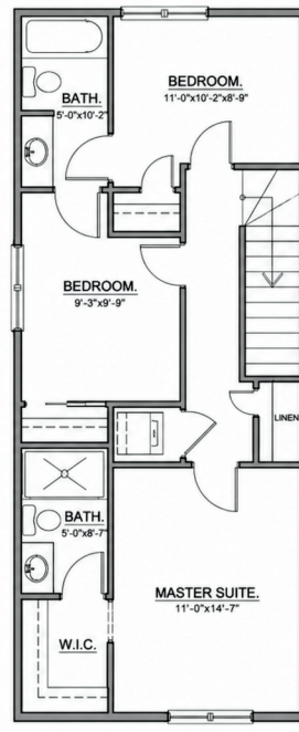
UPPER FLOOR 720 SQ.FT.
