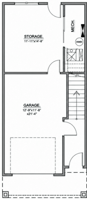
LOWER FLOOR 53 SQ.FT. DEVELOPED ENTRANCE 277 SQ.FT. GARAGE
