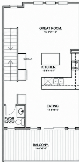
MAIN FLOOR 635 SQFT.
