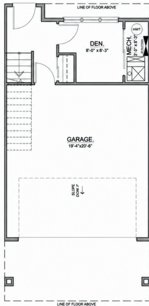
LOWER FLOOR 144 SQFT. DEVELOPED 422 SQFT. GARAGE
