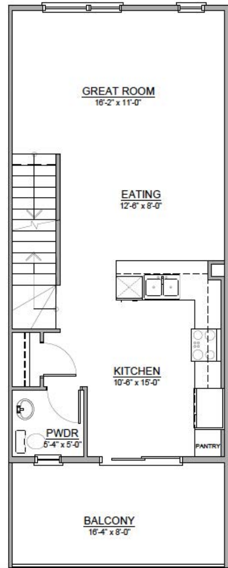
MODEL 4 MAIN FLOOR PLAN A
