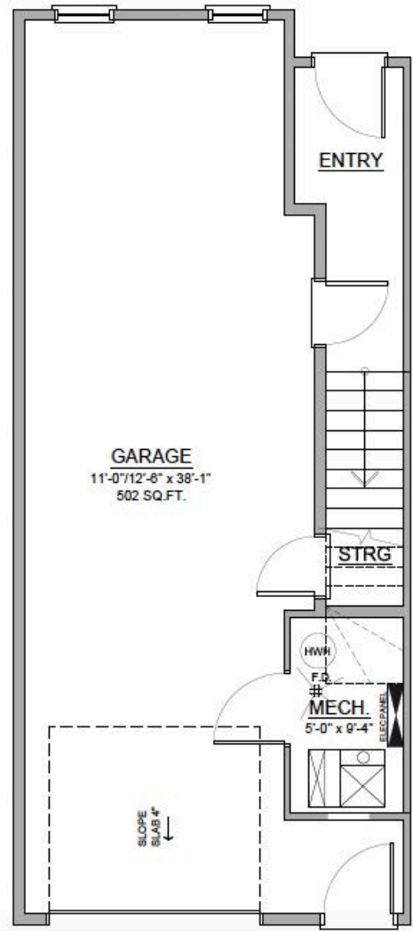
MODEL 1 LOWER FLOOR PLAN
