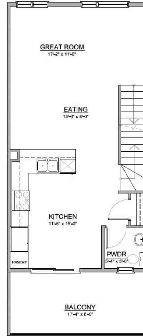
MODEL 3 MAIN FLOOR PLAN B (9'-1" CEILING HGT.) 609 SQ.FT. 1352 SQ.FT. TOTAL
