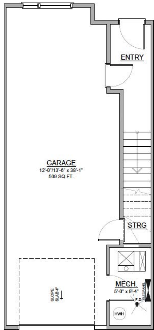
MODEL 3 LOWER FLOOR PLAN (9'-1" CEILING HGT.) 68 SQ.FT. DEVELOPED 509 SQ.FT. GARAGE
