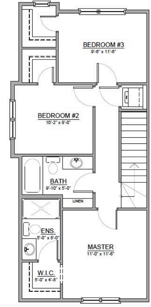
MODEL 1 UPPER FLOOR PLAN B
